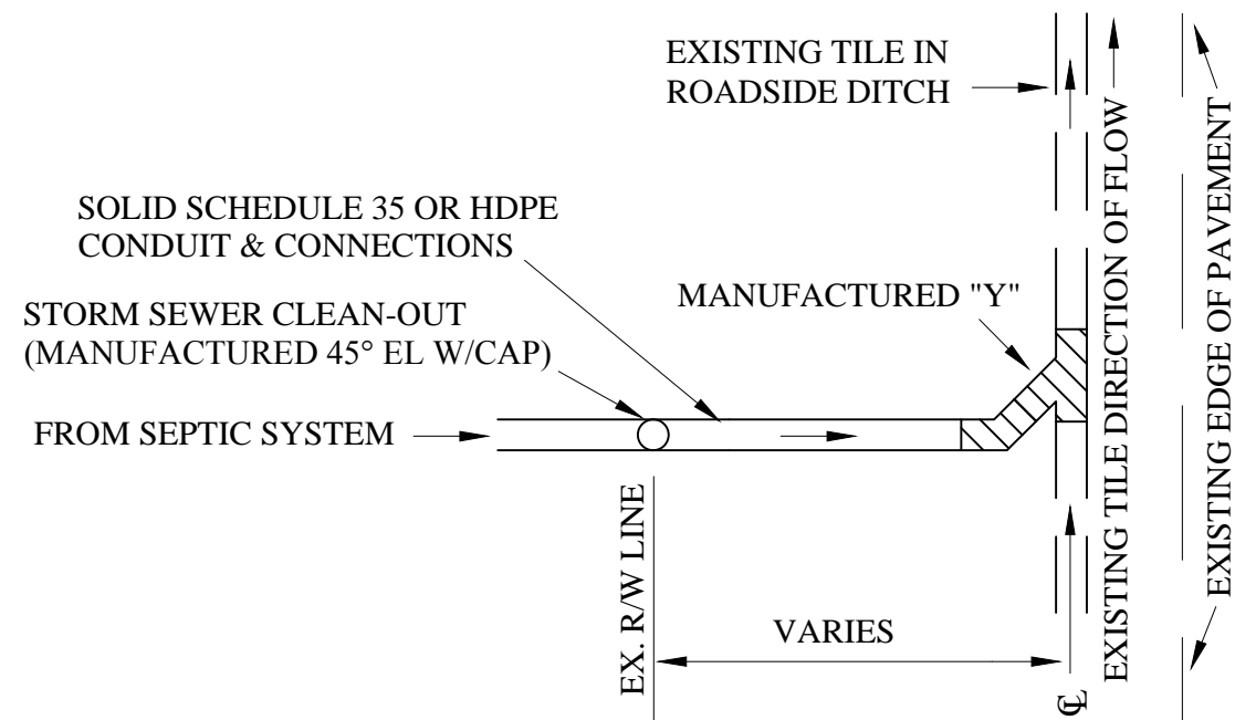
PLAN VIEW
