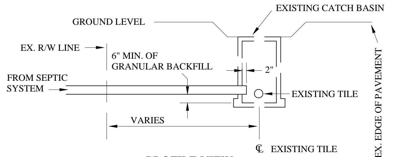
PROFILE VIEW
