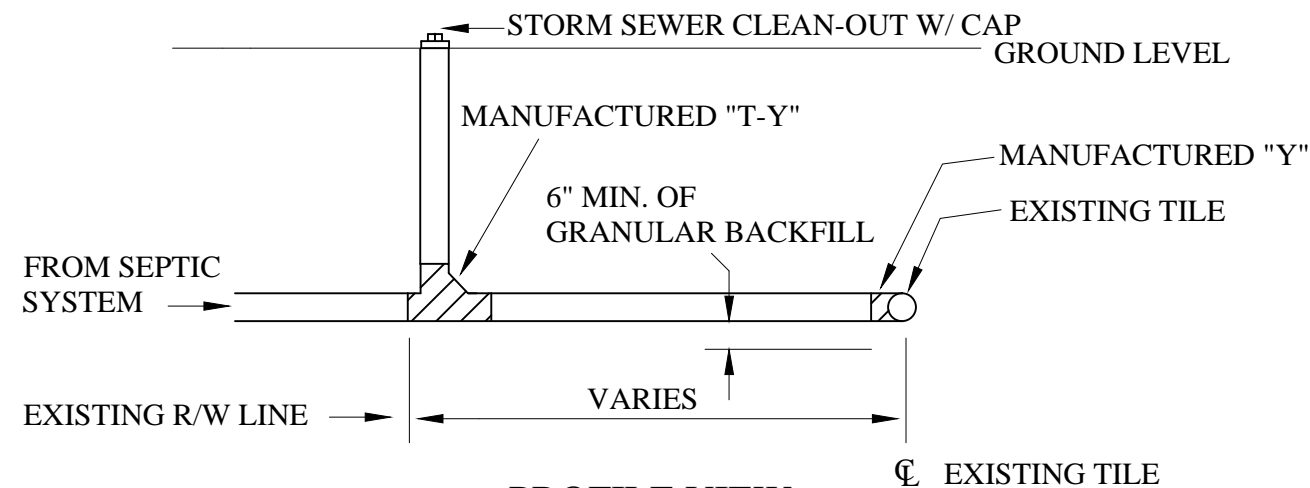
PROFILE VIEW
